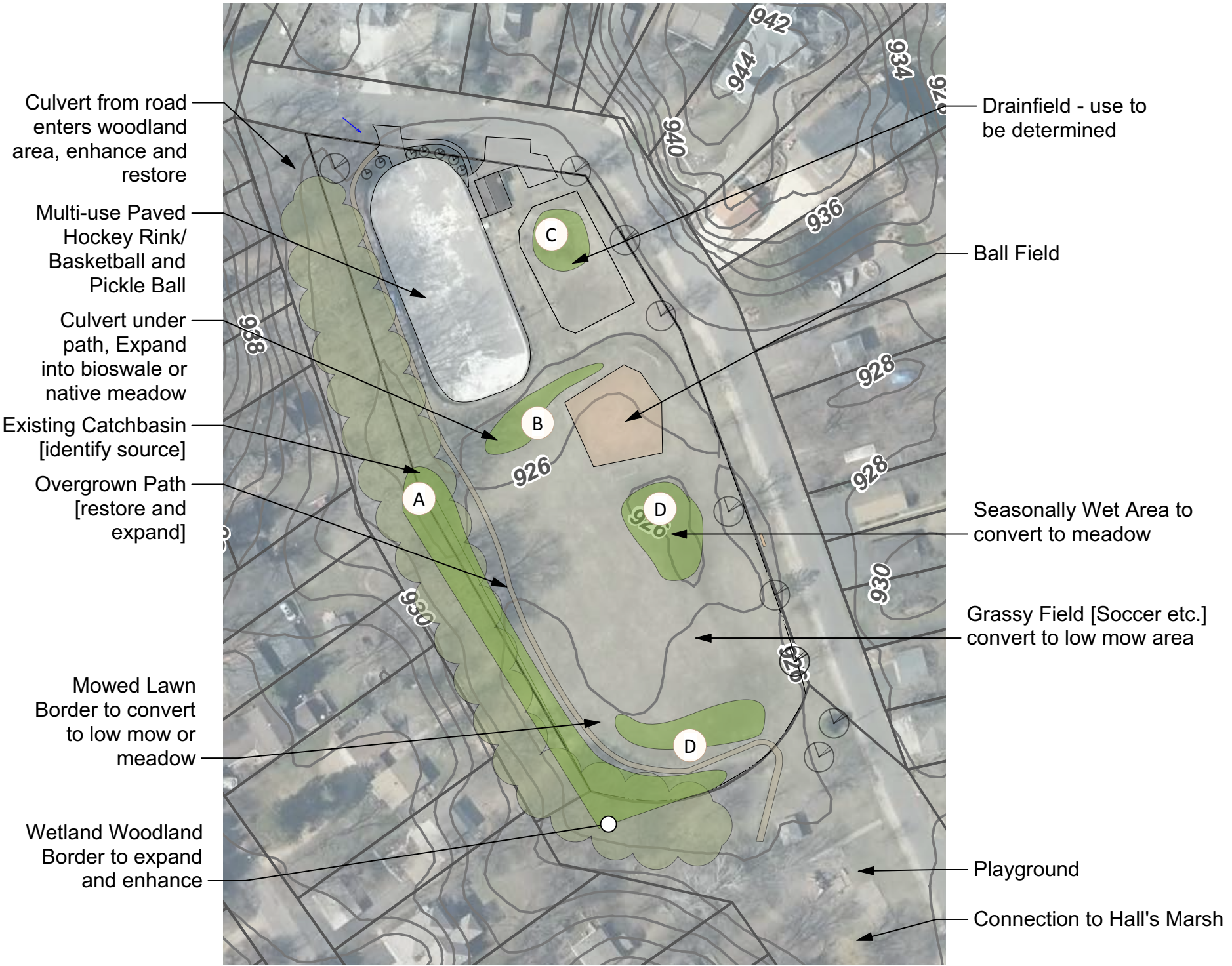
1 Project Overview Scale: 1" = 100'-0" 0 25 50 100 150 200 Feet
